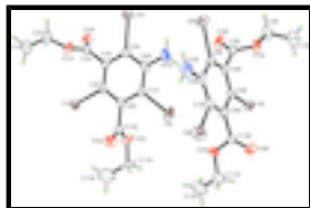
Fig. 1. A view of the two molecules of the title compound with the atomic numbering scheme. Displacement ellipsoids were drawn at the 50% probability level.
